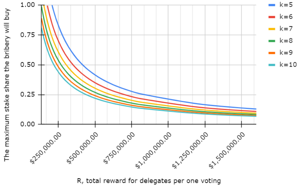
Fig. 1. Dependency of the maximum stake share that bribery can buy to have a Nash equilibrium in (B_2, S_2) on R , the total reward for delegates per voting round (for different k )
